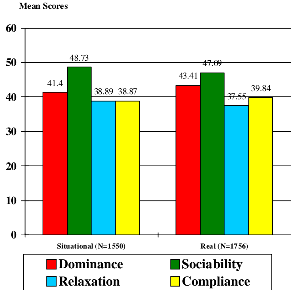
Dimension Scores
