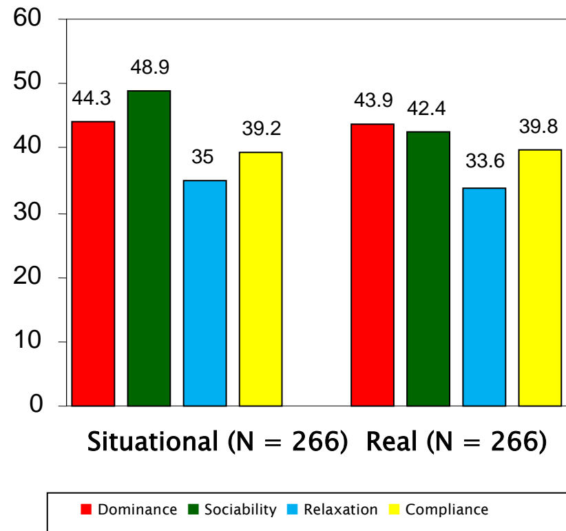
Mean Scores
