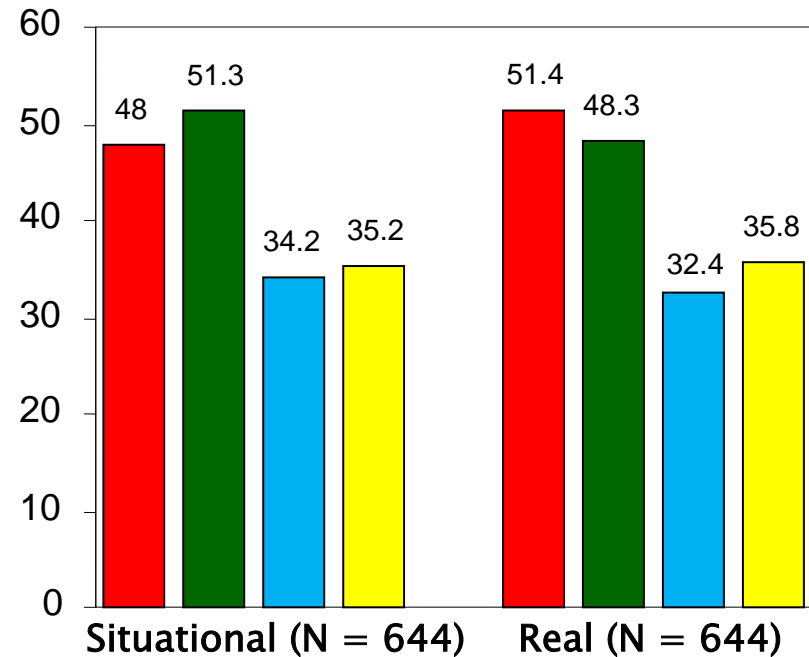
Mean Scores
