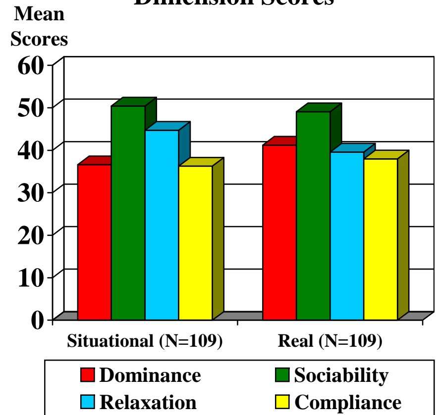
Dimension Scores
