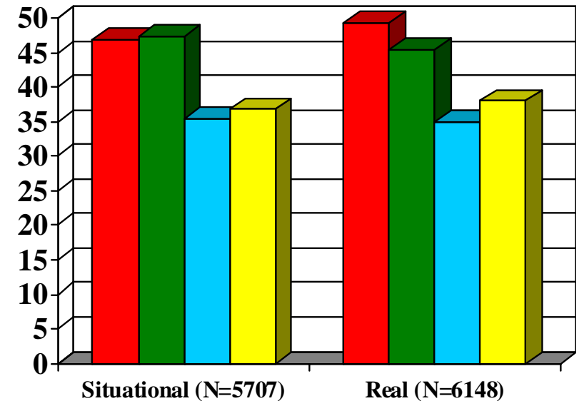
Mean Scores
